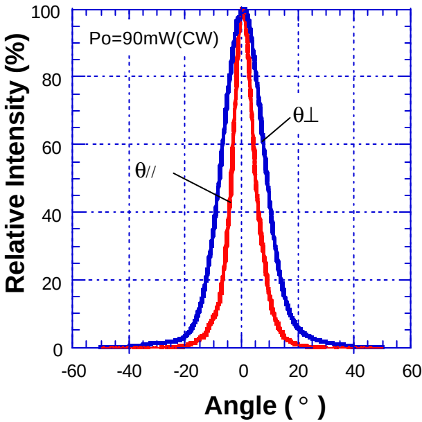
Far-Field-Patterns
